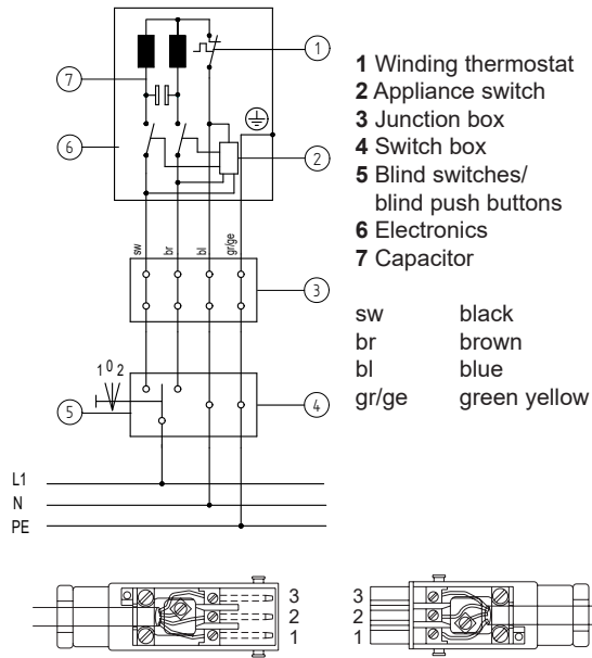
Fig. 5 Circuit diagram RoI Top D+ 230 V / 50 Hz and wiring with delivery with Hirschmann plug STAS 3
